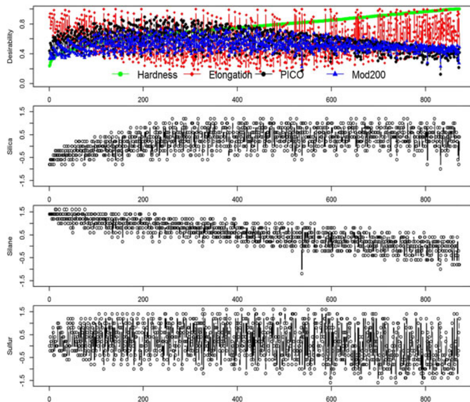
Figure B.1. The trade-off plot for the 872 locations on the PF of the mean models sorted primarily based on hardness
