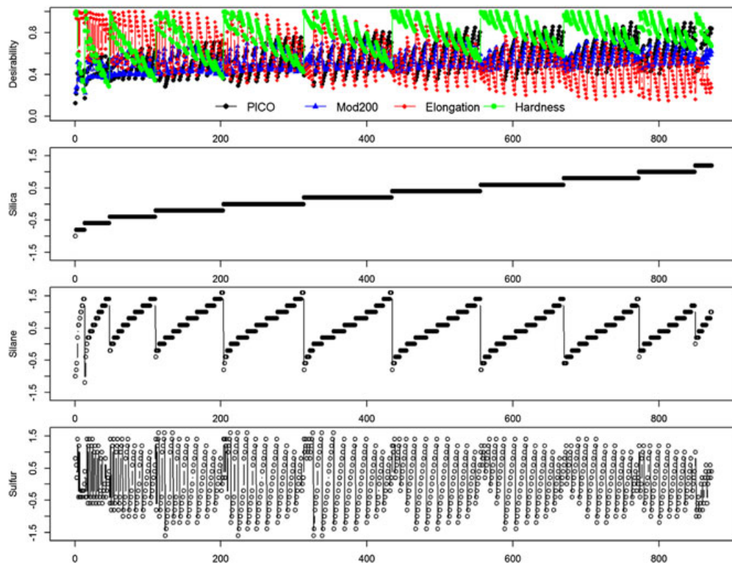
Figure 2. The trade-off plot sorted by the input factor values for silica, silane, and then sulfur
