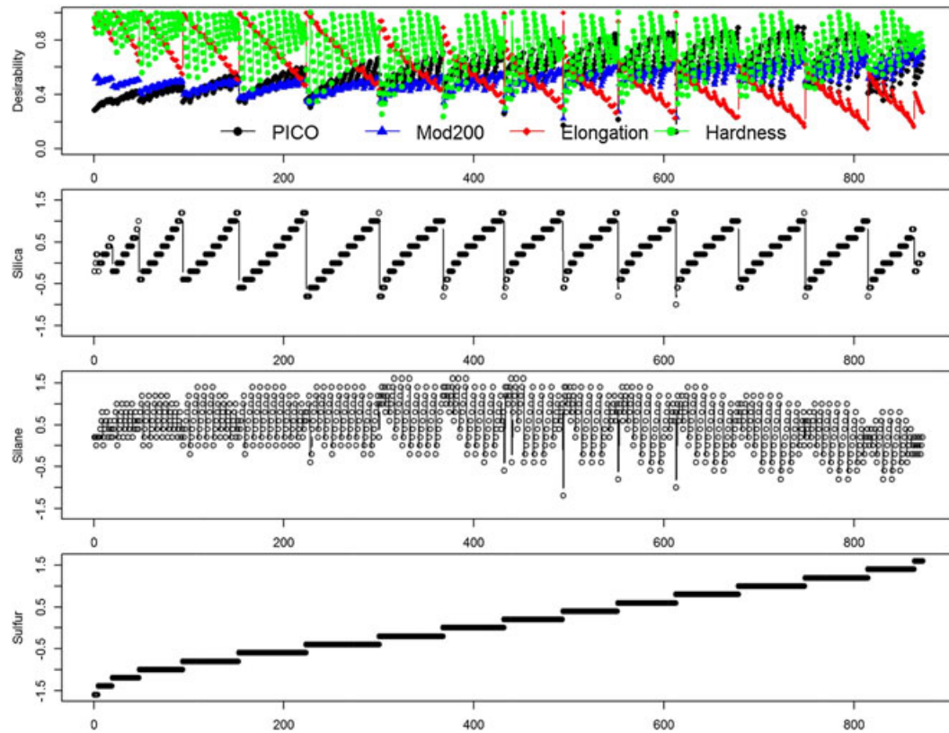
Figure B.2. The trade-off plot of the PF sorted primarily based on the input factor sulfur
