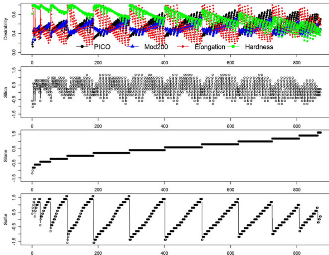
Figure B.3. The trade-off plot of the PF sorted primarily based on the input factor silane
